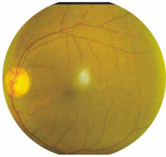
Normal Retina
